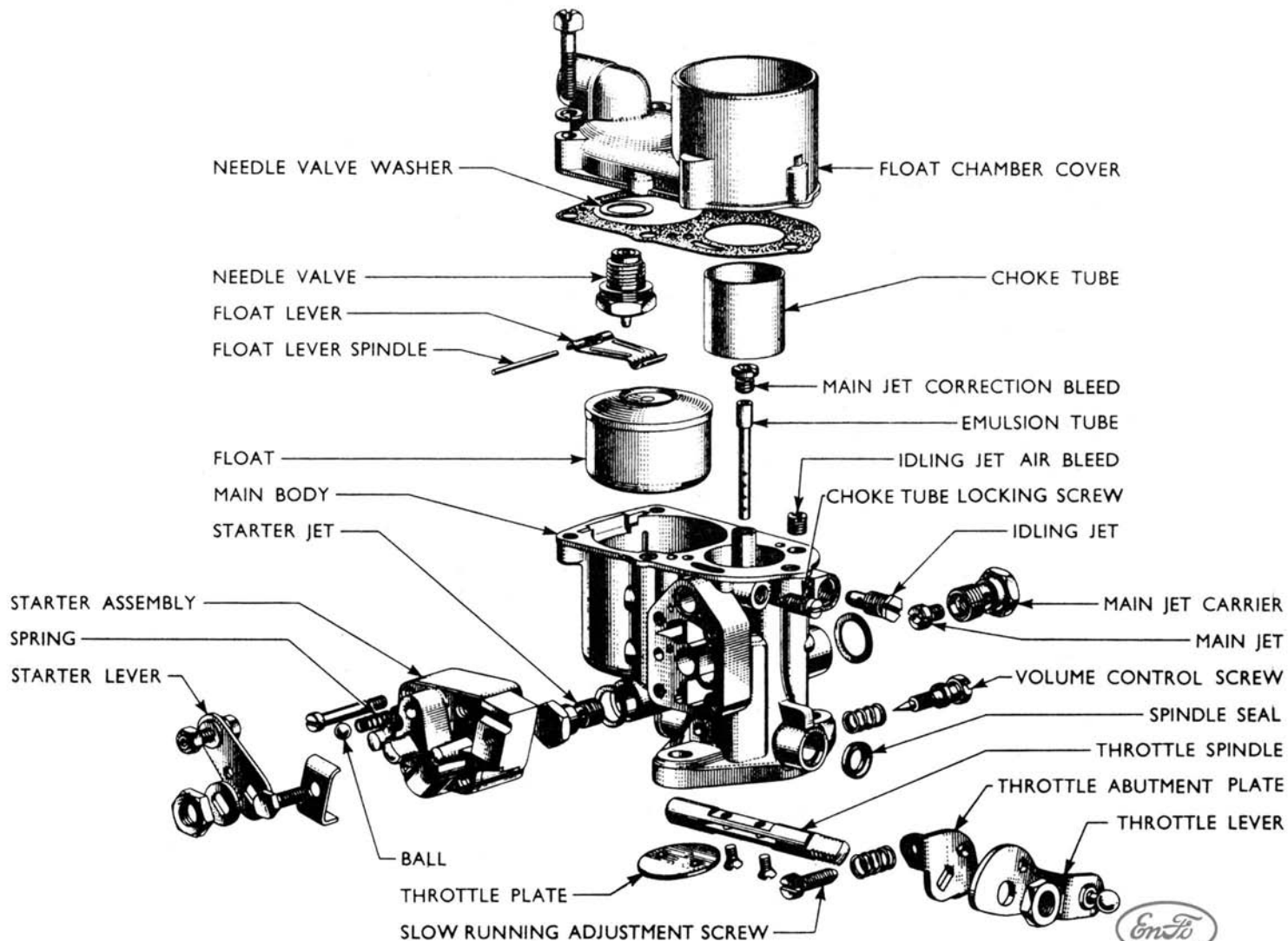
Exploded view of the B26.ZIC-2 carburetor used on the Anglia and Prefect.
