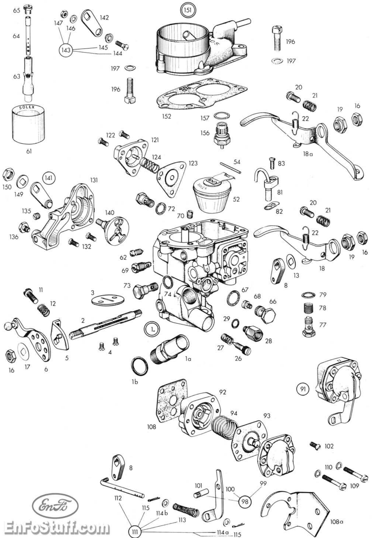
Exploded view of the Solex 32 PICBA carburetor used on the Taunus 17M.
