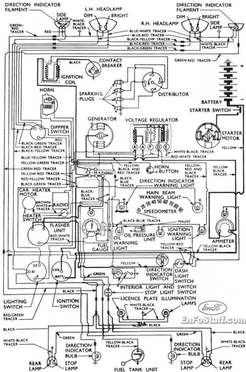
CONSUL WIRING DIAGRAM (AFTER OCTOBER, 1953)
