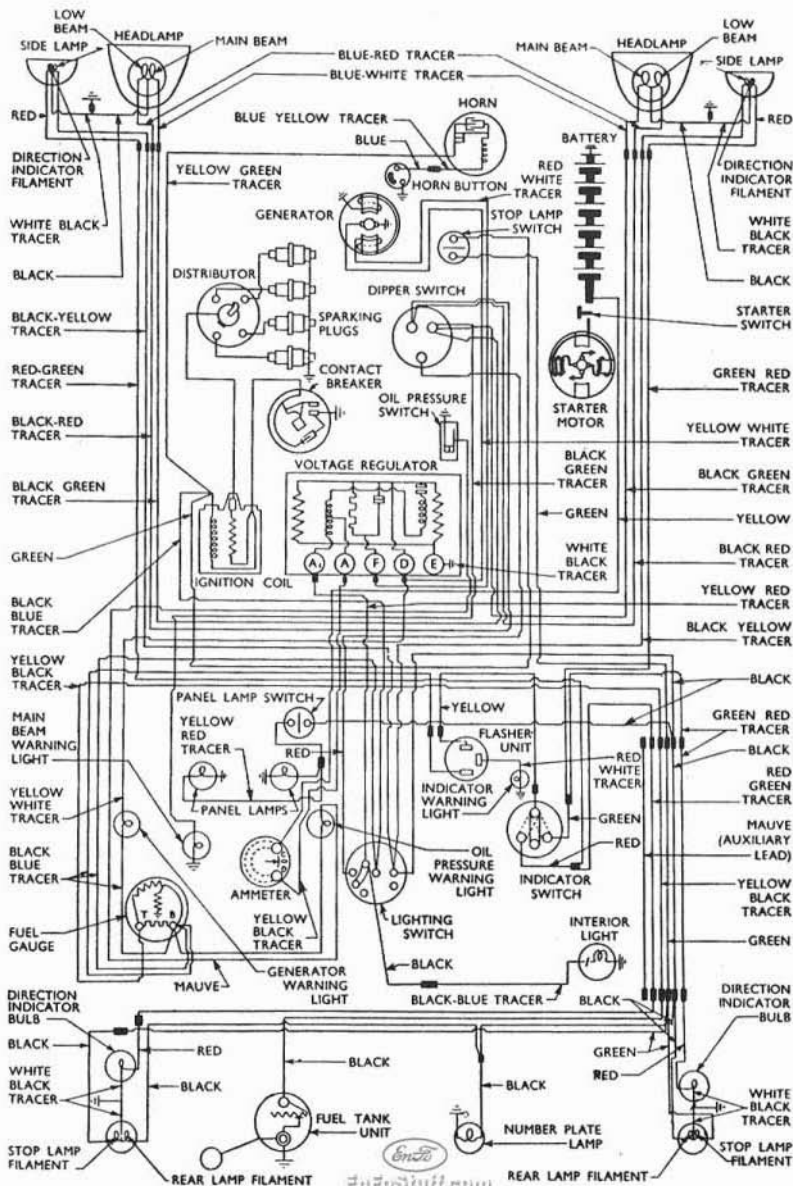
WIRING DIAGRAM FOR EARLY ANGLIA
