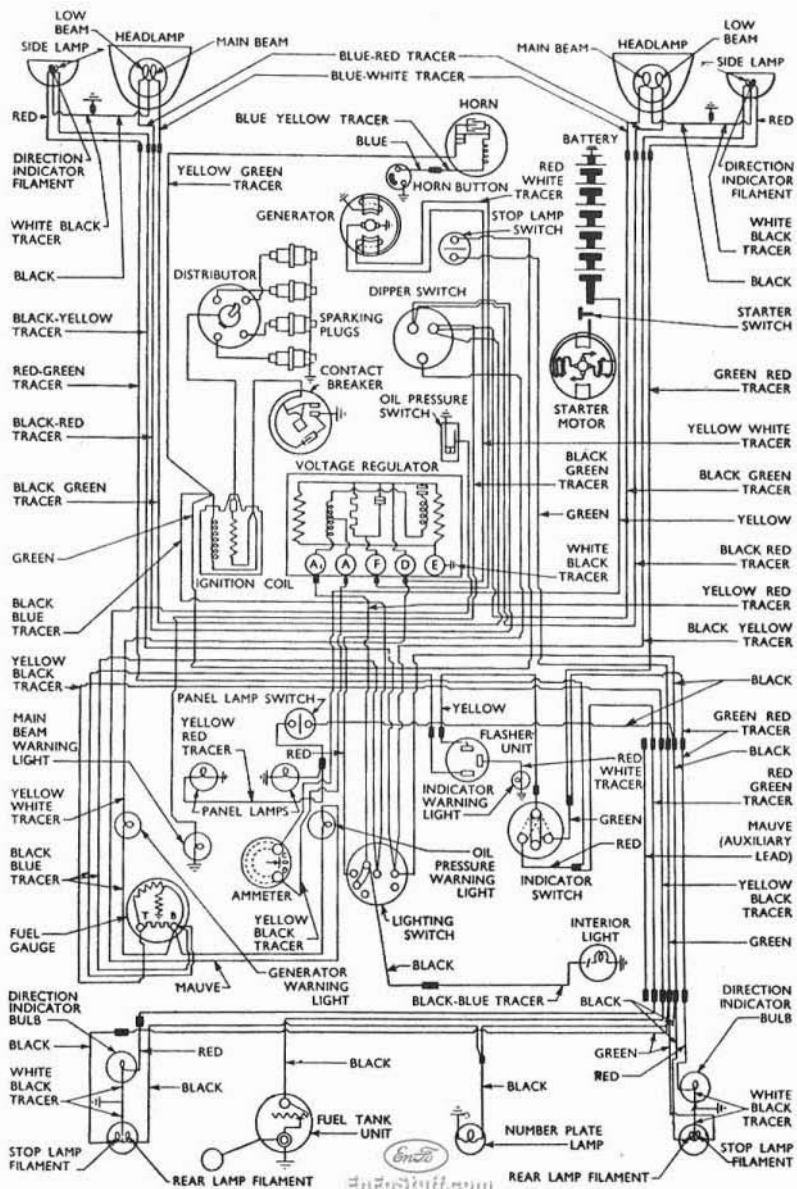
WIRING DIAGRAM FOR EARLY ANGLIA
