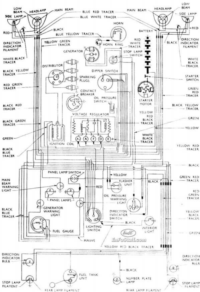
WIRING DIAGRAM FOR EARLY PREFECT
