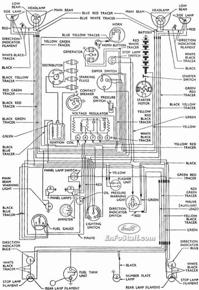
WIRING DIAGRAM FOR LATE ANGLIA, ESCORT AND 5-CWT VAN
