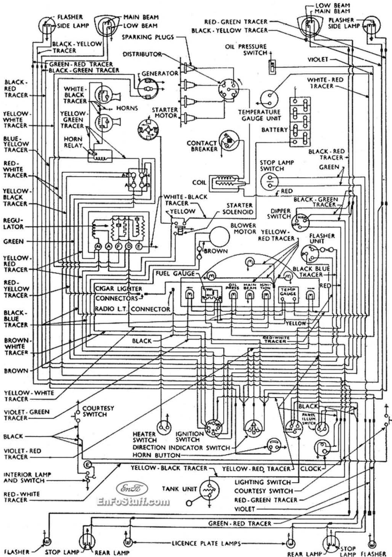
WIRING DIAGRAM FOR MARK II CONSUL
