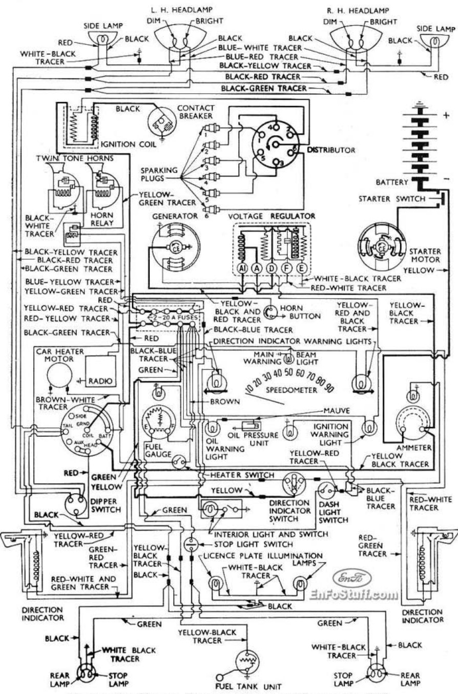
ZEPHYR-SIX WIRING DIAGRAM PRIOR TO SEPTEMBER, 1952
