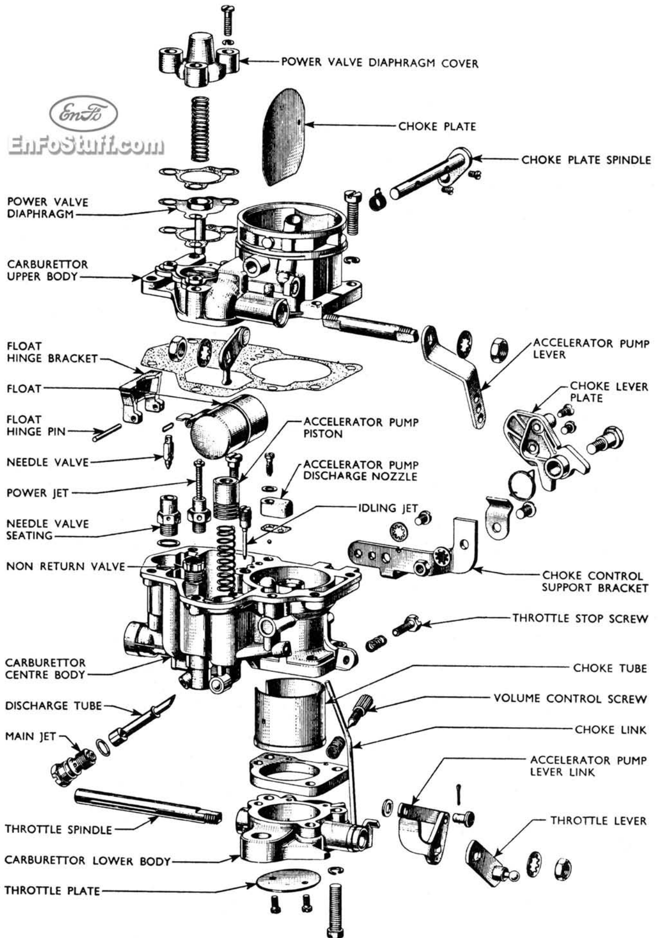
Exploded view of the carburetor used on the Consul, Zephyr, and Zodiac 1956-61.
