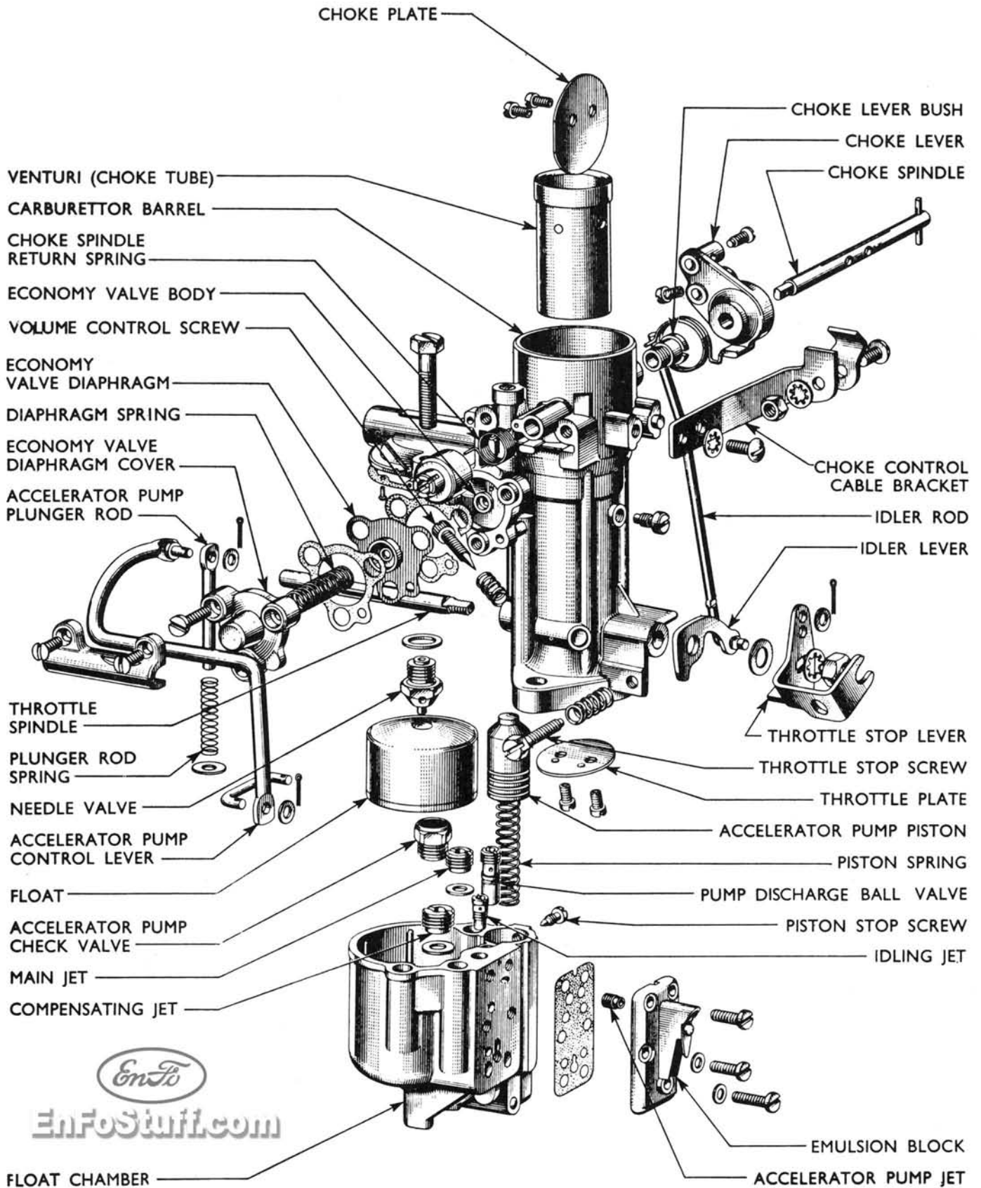
Exploded view of the carburetor used on the Consul, Zephyr, and Zodiac before 1956.
