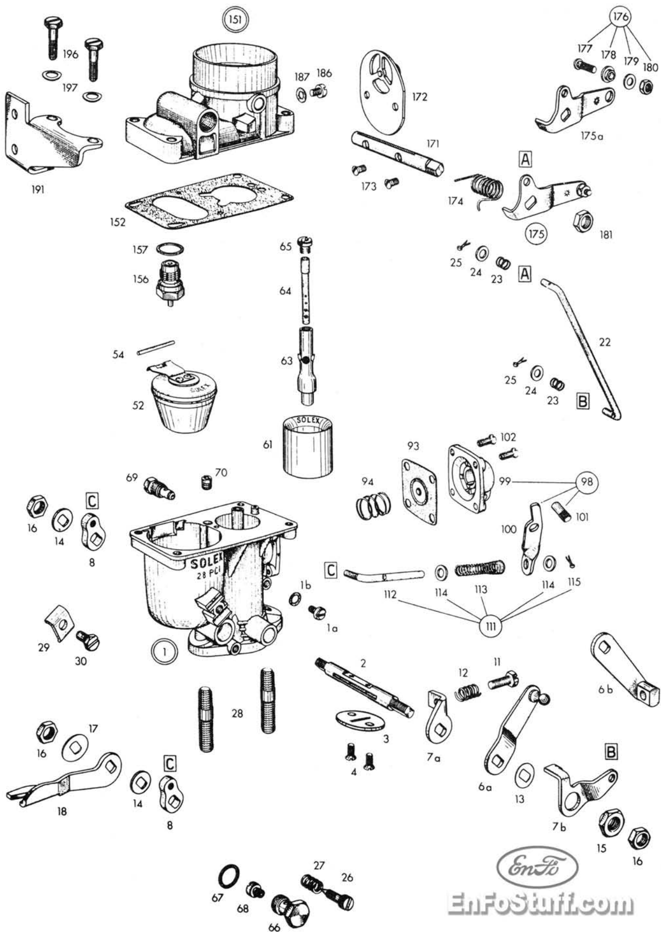
Exploded view of the Solex 28 PCI carburetor used on the Ford Taurus 12M.
