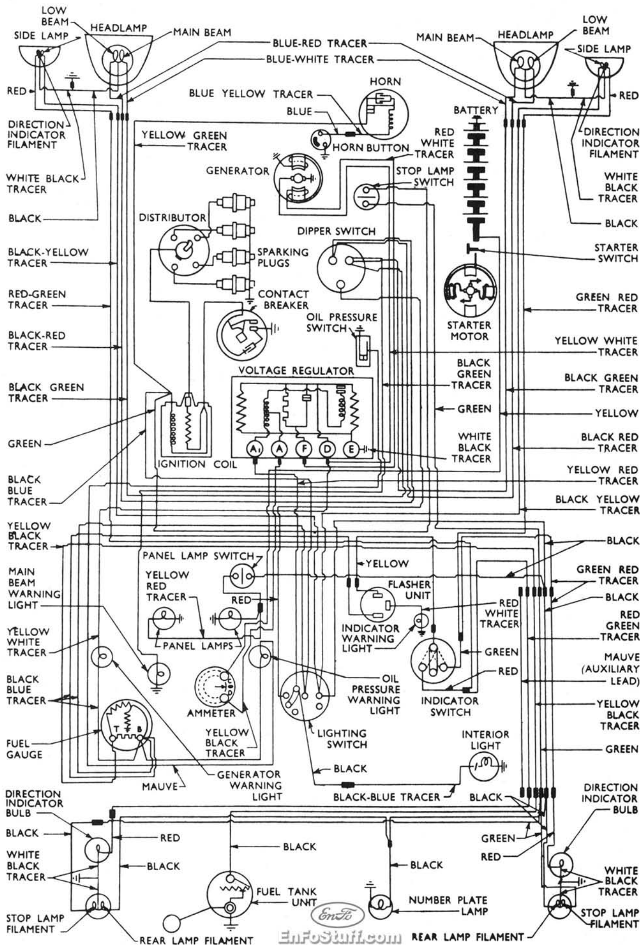
Chassis wiring diagram, Anglia 1953-57.
