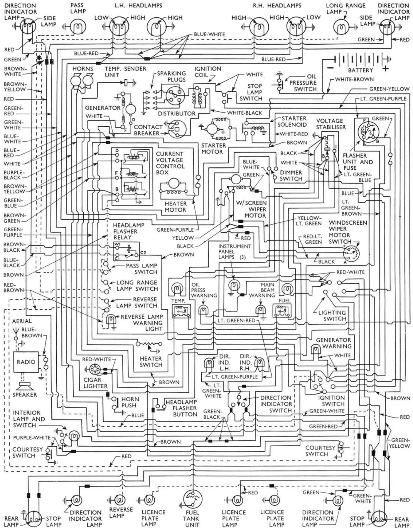
Chassis wiring diagram, Consul 315.
