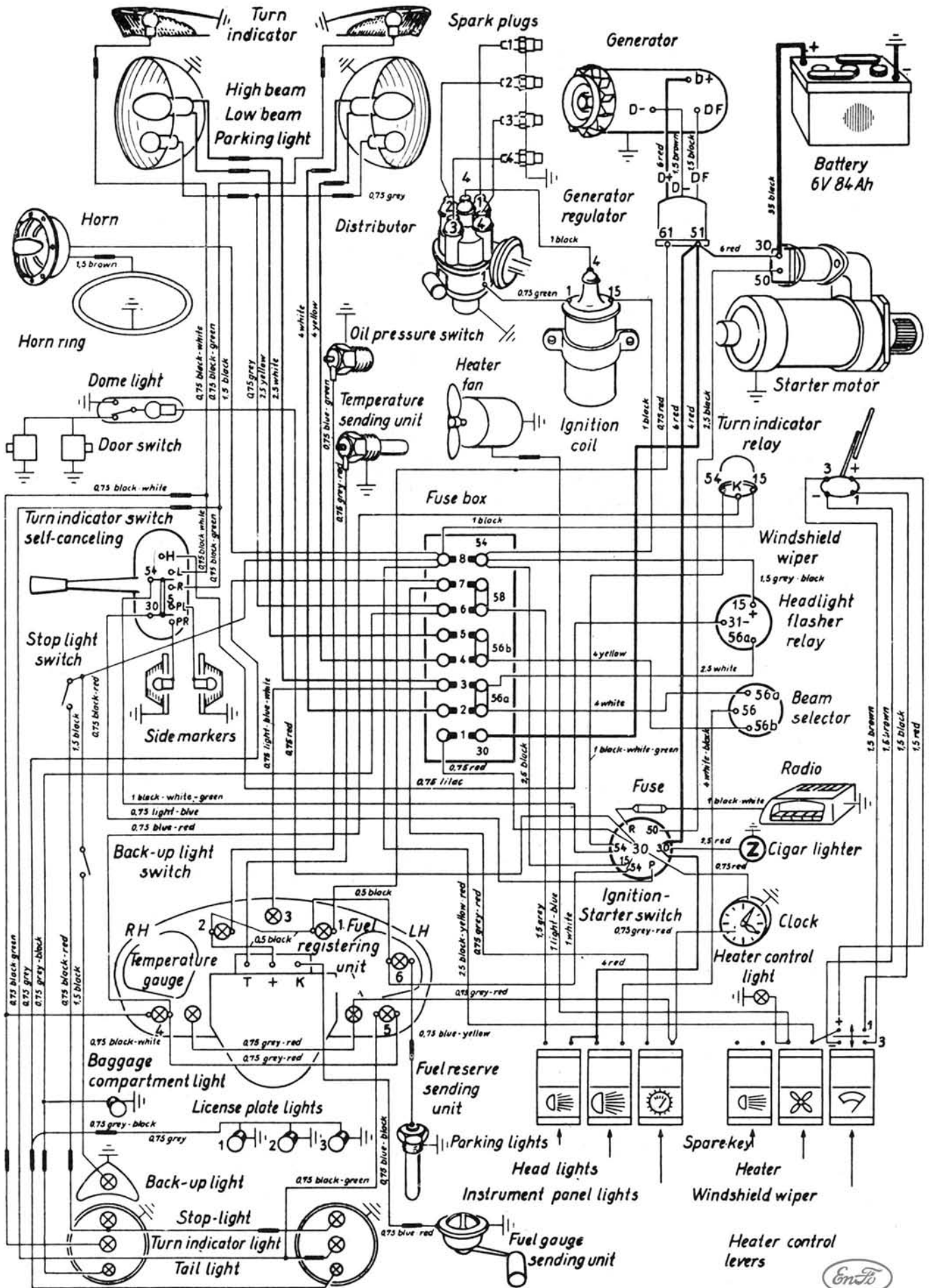
Chassis wiring diagram of the Taunus 12M, 12M Super, and 17M models.
