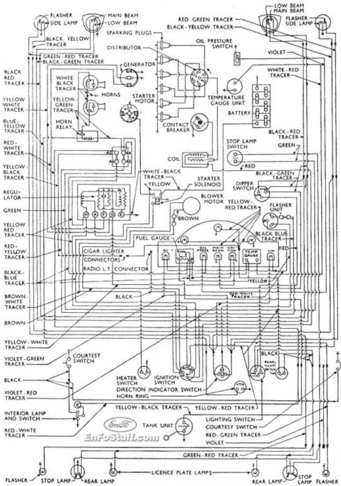
WIRING DIAGRAM FOR MARK II ZEPHYR AND ZODIAC
